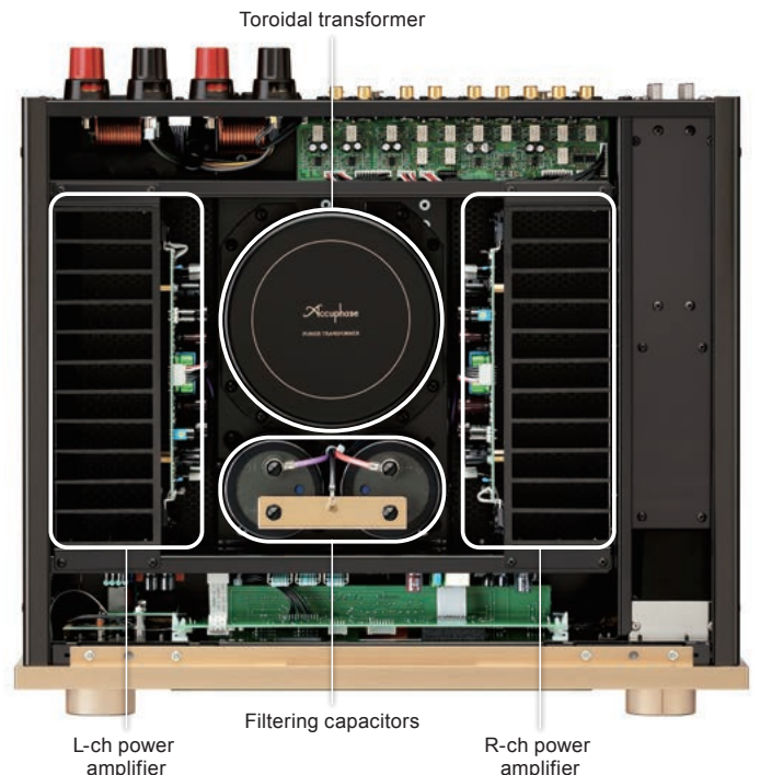
Toroidal transformer
