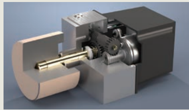
Volume sensor construction
