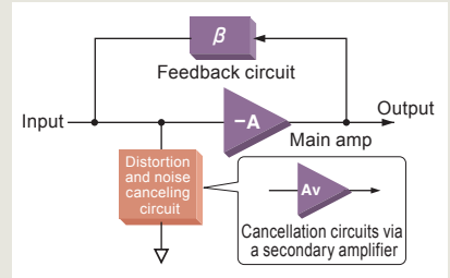
Block diagram of ANCC
